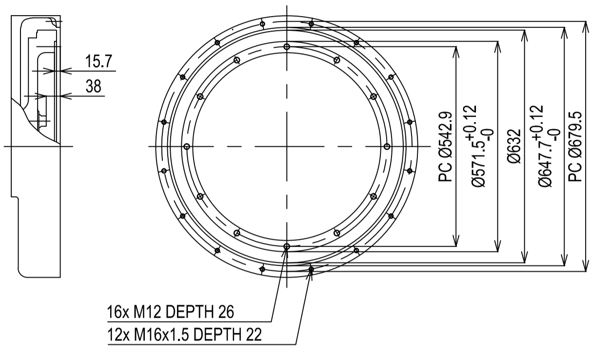
Flywheel housing & Flywheel : SAE #0 & #18
