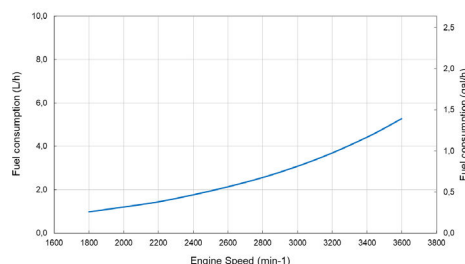
3YM20 Fuel consumption (propload exp 3.0)
