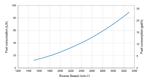
6LY440 Fuel consumption (load exp. 2.5)
