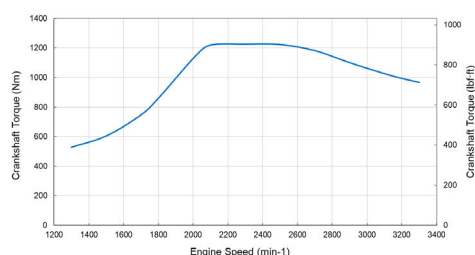
6LY440 Torque curve
