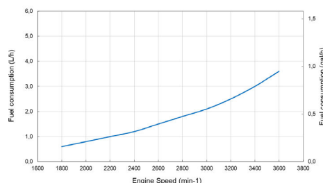
2YM15 Fuel consumption (propload exp 3.0)
