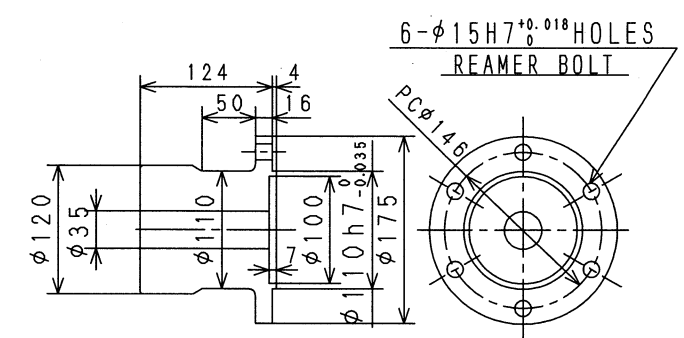
Ⓑ COUPLING OF OUTPUT SHAFT (SCALE 1/5)
