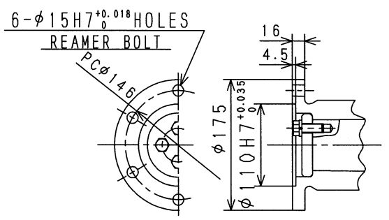
Ⓐ COUPLING OF PROPELLER SHAFT (SCALE 1/5)
